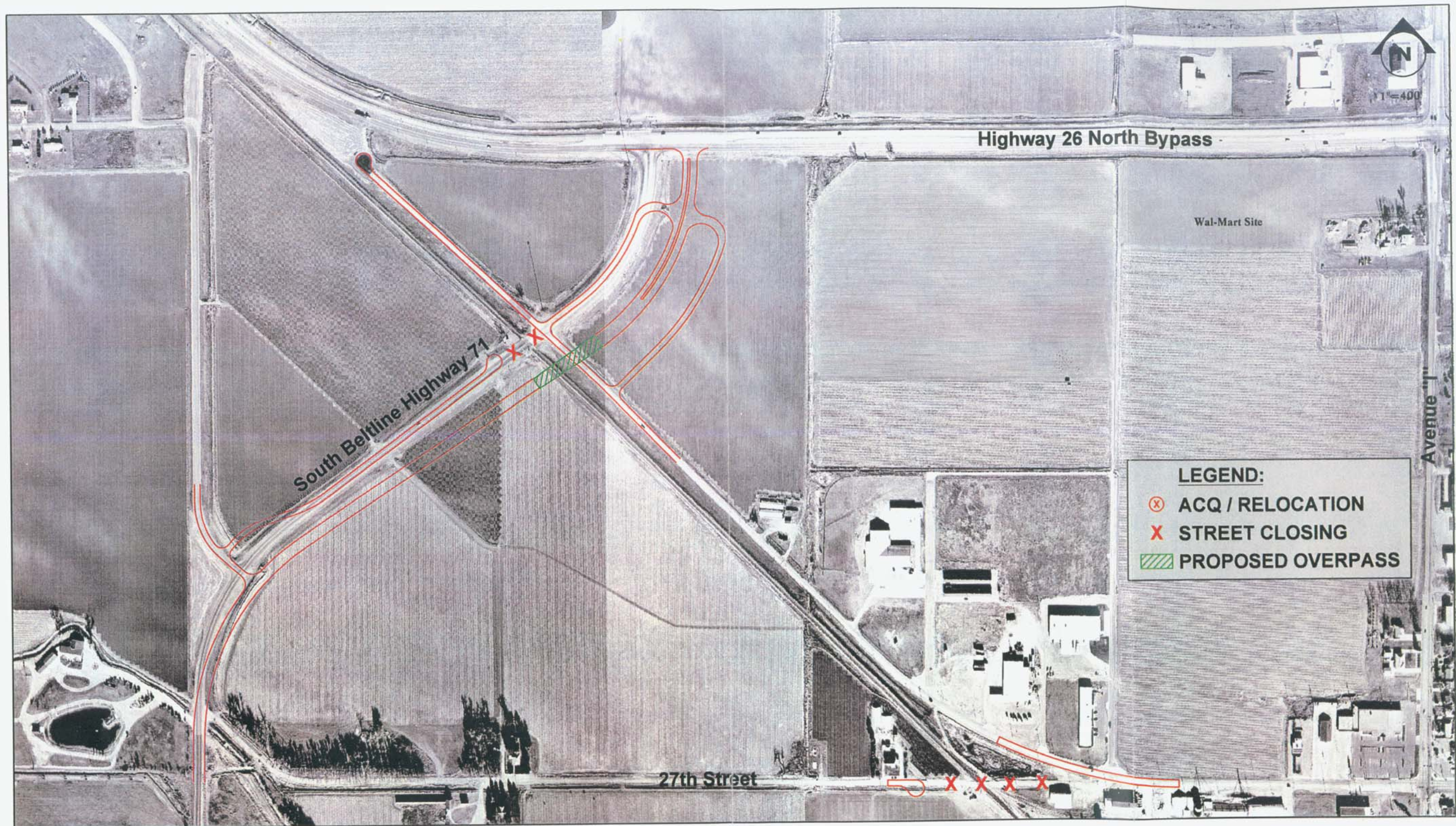
Figure 9 Alternate 1 - South Beltline Hwy. 71 Overpass Page 22
